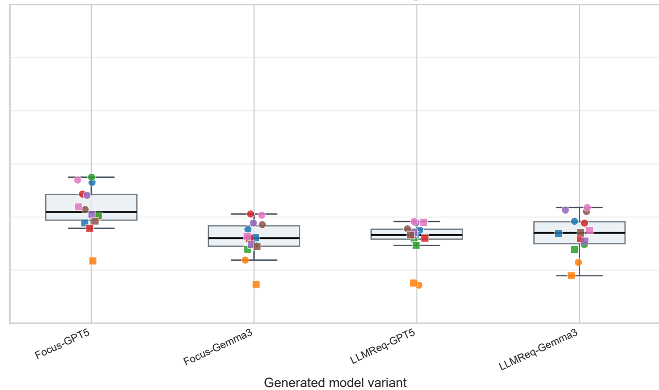
Backward all-candidate F1@3
